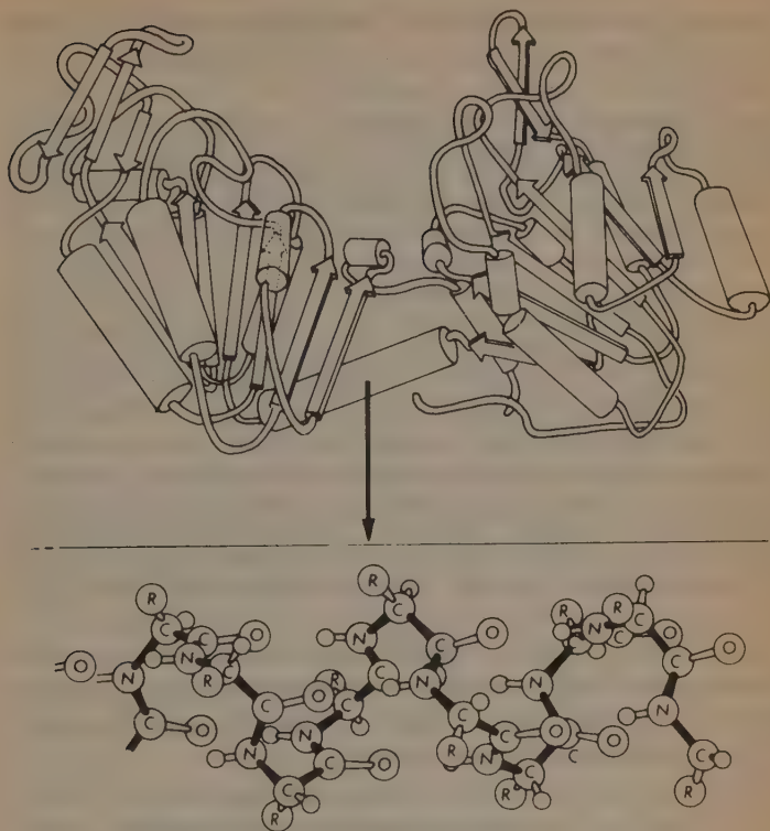
Figure 9 Above: The structure of the enzyme phosphoglycerate kinase, isolated from horse muscle. \alpha - helices are represented by cylinders and \beta - strands by arrows. Below: The structure of an \alpha - helical region in more detail. (After Banks et al. , 1979.)
