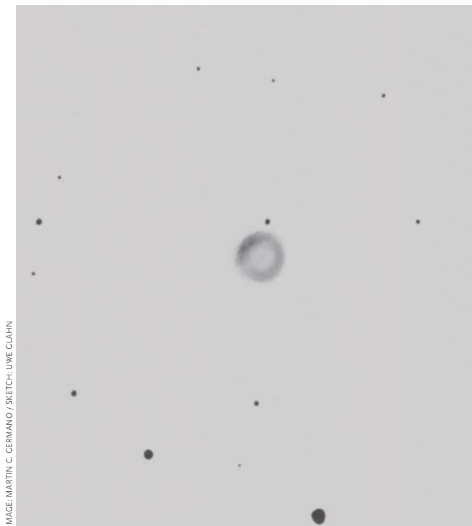
THE OTHER RING Below left: The faint star at the north edge of M 1-64 shows in this sketch made at 586x with a 27-inch reflector. Right: A 14.5-inch reflector reveals M 1-64's ring structure.
