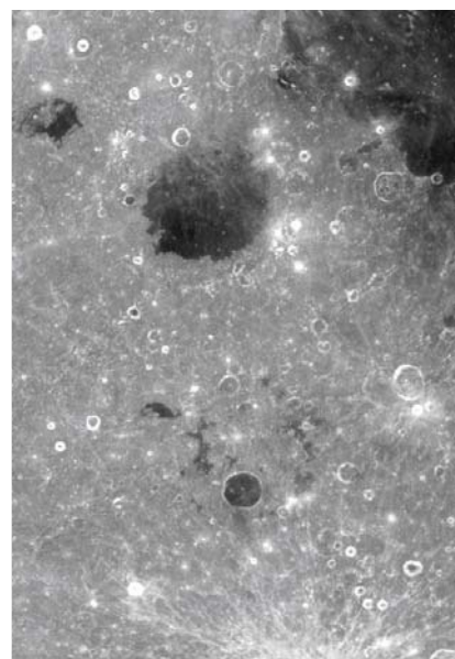
The Crüger-Sirsalis impact basin, south of Grimaldi along the Moon's western limb, shows no rims. Yet its gravity signature (center) and telltale patches of mare lava seen near full Moon (right) confirm its reality.
